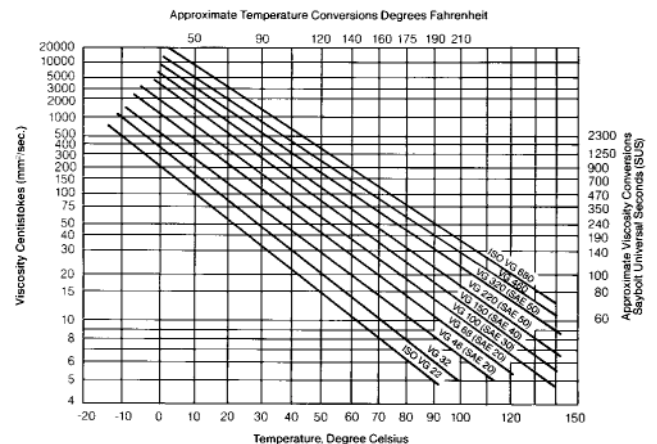
Figure 2 Viscosity-Temperature Chart
