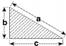
Right-angled Triangle
