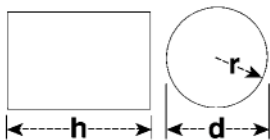
Cylinder
