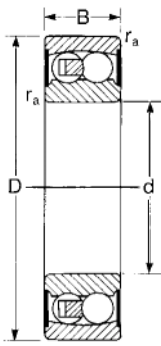
Cylindrical bore
