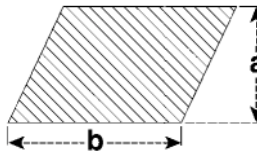
Parallelogram
