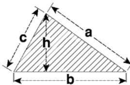
Acute-angled triangle
