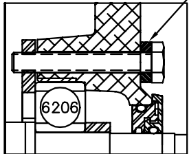
PULLEY END DETAIL
